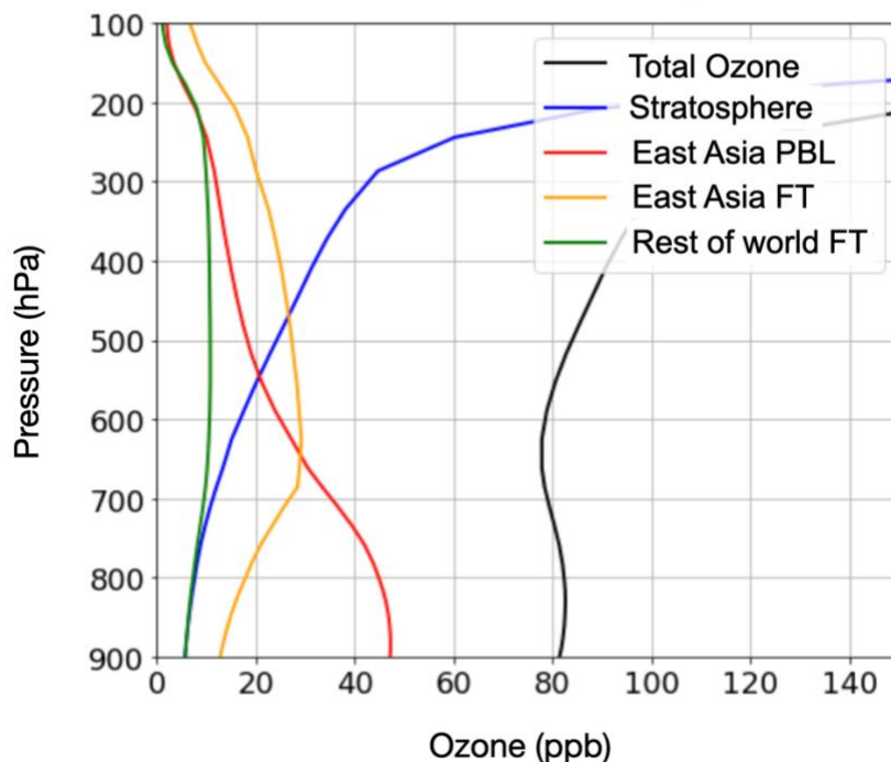
Figure 6 Source attribution of mean ozone over East Asia in May-June 2015-2019 as simulated by GEOS-Chem.
