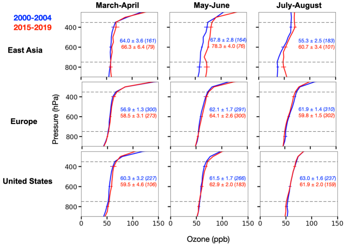
80 Figure 1 Mean IAGOS vertical profiles of ozone mixing ratios over East Asia (30.0-45.0 ° N, 109.0-145.0 ° E), Europe (35.0-54.0 ° N, -11.0-30.0 ° E), and the United States (28.0-49.0 ° N, -124.6.0- -66.8 ° E) for 2000-2004 and 2015-2019. Average and standard deviations of ozone column mixing ratios in the free troposphere (750-350 hPa) are shown with numbers of profiles in italics. Horizontal bars are standard deviations for selected 25 hPa vertical pressure levels. Dashed lines are the 750 hPa and 350 hPa pressure levels defining the free troposphere for the purpose of our work. 85
