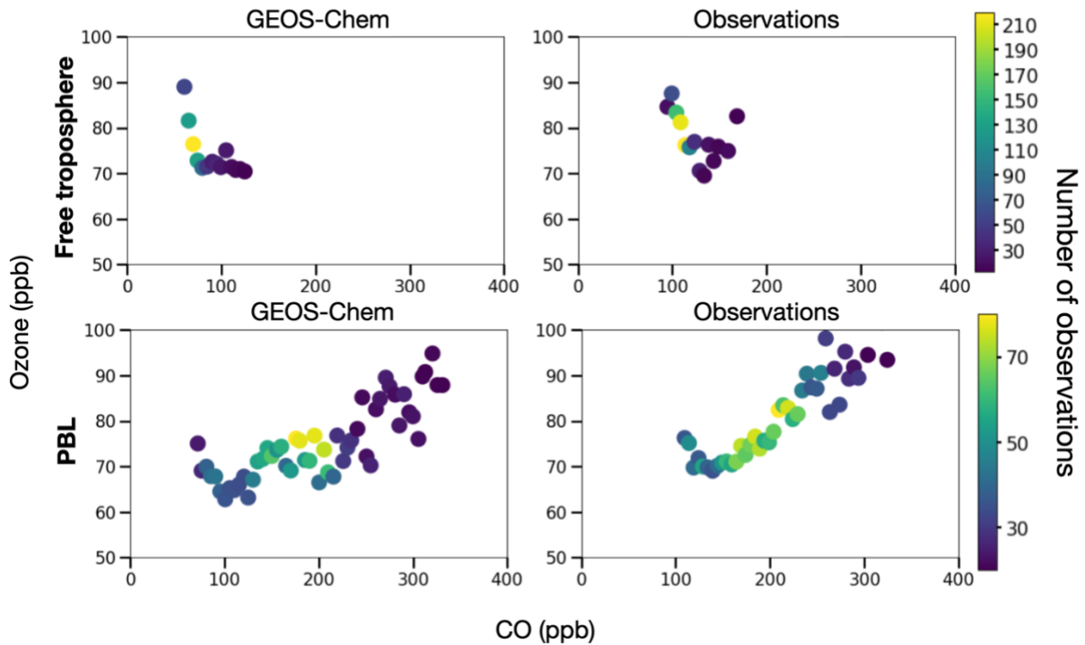
Figure 4 Ozone versus CO mixing ratios in the free troposphere (750-350 hPa) and PBL (surface -750 hPa) over and around the Korea peninsula during the KORUS-AQ aircraft campaign in May-June 2016. 1-minute observations are averaged over 5-ppb CO mixing ratio bins and compared to the GEOS-Chem simulation sampled along the aircraft tracks. Only bins with 20 or more observations are shown.
