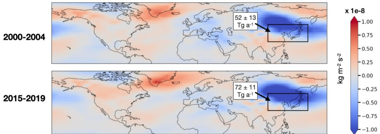
Figure 5 Annual mean vertical advective flux of ozone at 100 hPa, averaged for 2000-2004 and 2015-2019. Negative values (blue) indicate downward motion. Net downwelling rates over East Asia (30.0-45.0 ° N, 109.0-145.0 ° E) are shown inset with interannual standard deviations.
