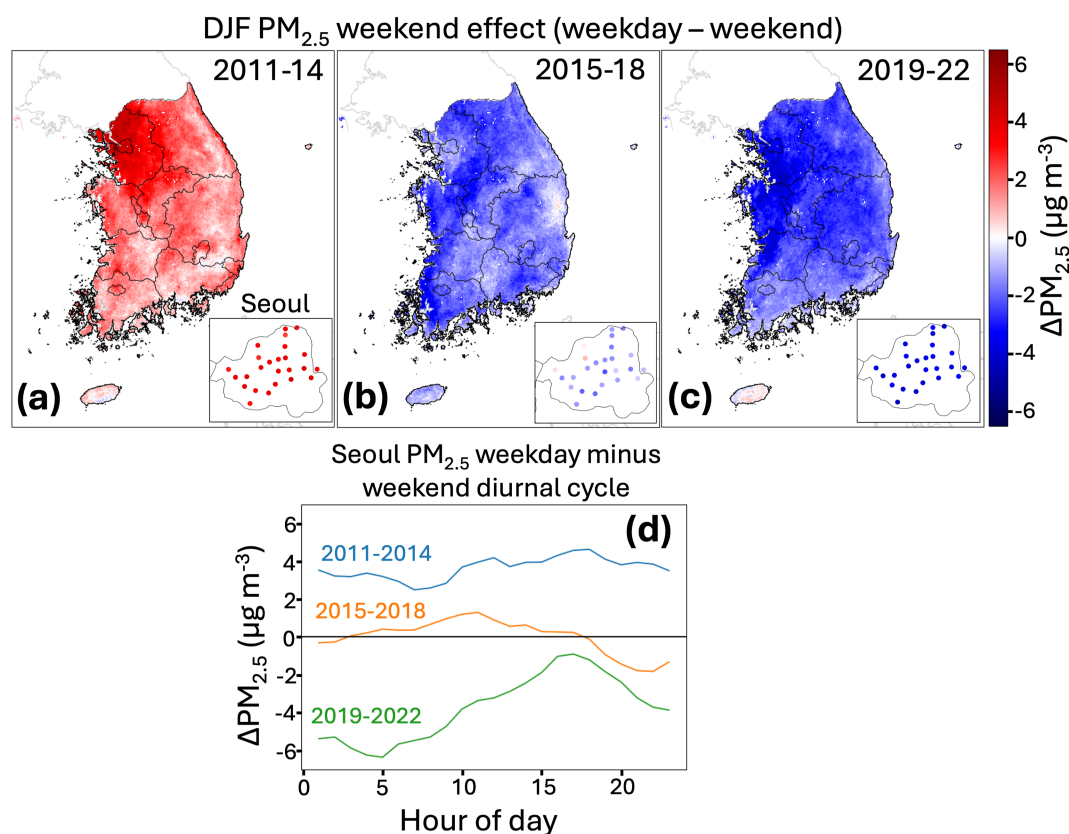
Figure 4. Wintertime (DJF) PM 2.5 weekend effect in South Korea. ΔPM 2.5 denotes the difference between mean weekday and weekend PM 2.5 concentrations. Panels (a) through (c) show maps of ΔPM 2.5 for (a) 2011–2014, (b) 2015–2018, and (c) 2019–2022, where red (positive ΔPM 2.5 ) indicates that weekdays are more polluted than weekends. PM 2.5 concentrations are inferred using machine learning from geostationary satellite AOD data (Pendergrass et al., 2025), except for Seoul (inset) where direct continuous measurements are available from sites through the 2011–2022 period. Panel (d) shows the diurnal variation of ΔPM 2.5 in Seoul for 2011–2014, 2015–2018, and 2019–2022.
