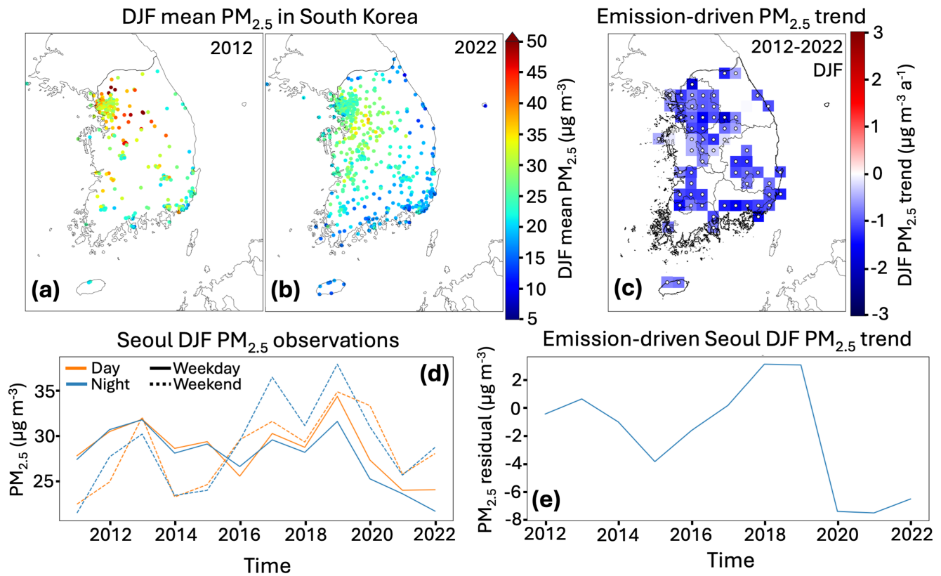
Figure 1. December–February (DJF) PM_{2.5} and trends in South Korea. Panels (a) and (b) show DJF mean PM_{2.5} at AirKorea surface stations in (a) 2012 and (b) 2022. PM_{2.5} monitoring at these stations started in 2015, and data for 2012 are produced using a random forest (RF) algorithm applied to the then-available station data including PM_{10} (Pendergrass et al., 2025). Panel (c) shows the DJF emission-driven trend in PM_{2.5} after removing meteorological influence with a multi-linear regression (MLR) fit. Panel (d) shows observed DJF PM_{2.5} averaged over 25 sites in the city of Seoul, disaggregated into daytime (8–18 LT) and nighttime (22–5 LT) for weekdays and weekends. Panel (e) shows the emission-driven PM_{2.5} timeseries (residual from the meteorological MLR model) for the Seoul 0.25^\circ \times 0.3125^\circ grid cell (centered at 37.5^\circ N , 127.0^\circ E ) and averaging data from 37 sites.
